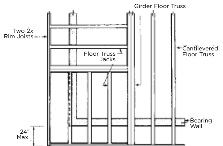
Floor Cantilevered Perpendicular and Parallel to Floor Truss Span
